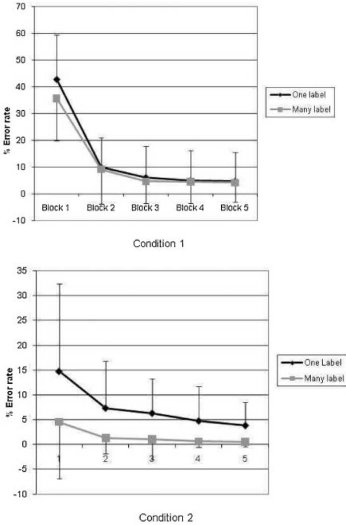
Figure 1. Acquisition curves for the associations with the one and many labels for the two conditions. Error bars denote 1 SD; for clarity, we show only positive error bars for the one-label curves and only negative error bars for the many-label curves
